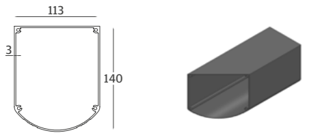
3 Carrier Post Profile
