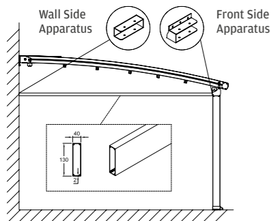
Side Beam Profile
