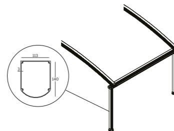
Additional Carrier Post Profile
