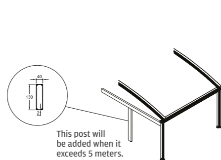
Additional Side Post and Beam Profile
