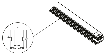
Additional Rafter Profile
