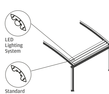
Aerofoil Louvre Profile
