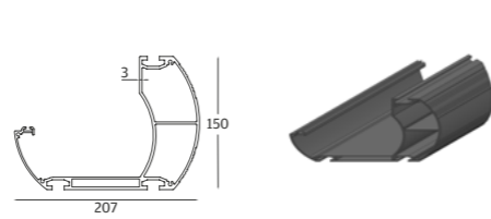
2 Gutter Profile
