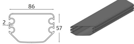
6 Motor Box Profile
