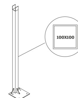
Additional Carrier Post
